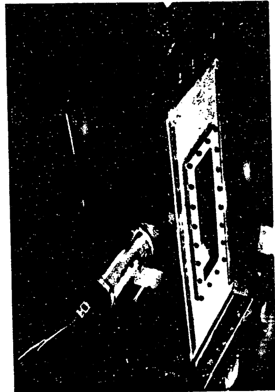
Apparatus for detailed velocity field mapping of the wake phenomena around a cylinder subject to random oscillatory flows.
